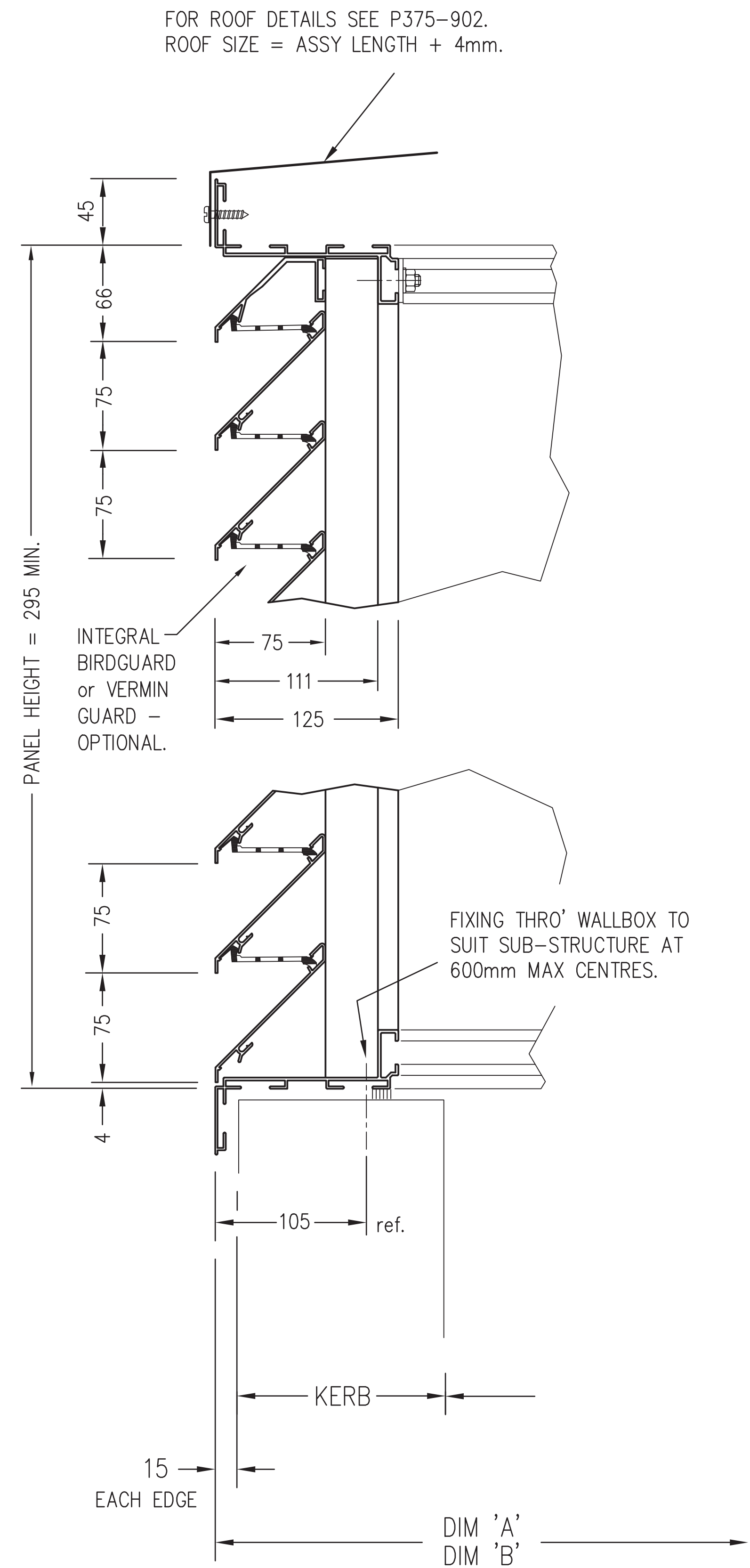
VERTICAL SECTION THRO'
